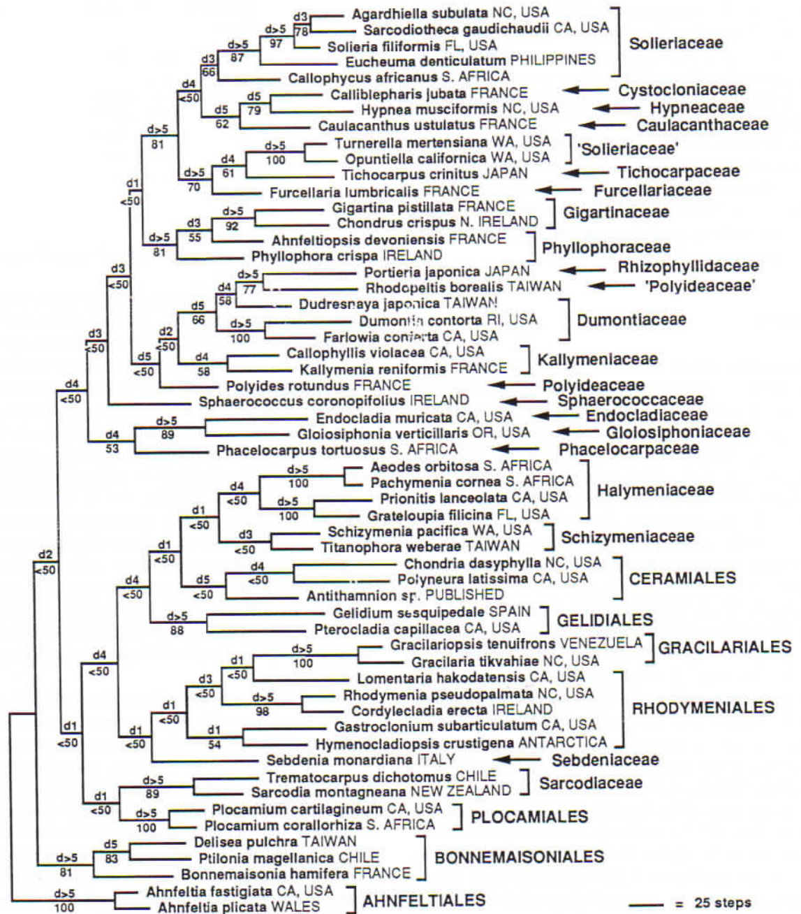
Figure 1. Single maximum parsimony tree of length = 4315, CI = 0.213 and RI = 0.384, resulting from a multiple heuristic search analysis of rbcL sequence data from 57 red algal species. Decay indices are indicated above and bootstrap values (%) below branches. Branch lengths are proportional to estimated mutational steps.
